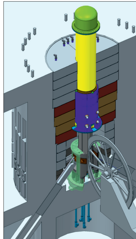
Schematic view of IBR-3
