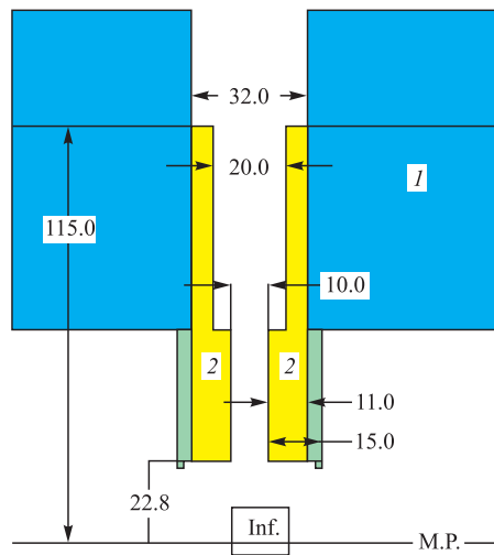
Fig. 3. Central plug cross section: 1 — pole; 2 — movable part
