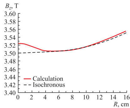
Fig. 4. Mean magnetic field
