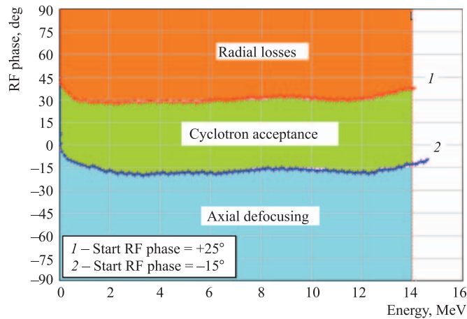
Fig. 18. RF phase excursion vs. the energy
