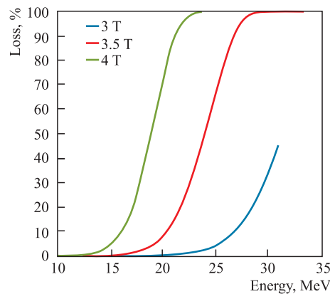
Fig. 19 (color online). H^- magnetic stripping, energy gain 40 keV/turn
