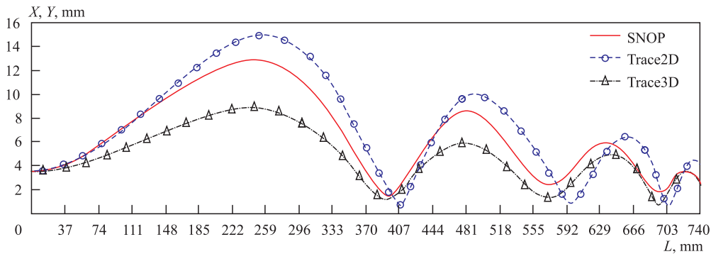
Fig. 9. SNOP/Trace2D/Trace3D results for the 15-mA beam from the ion source
