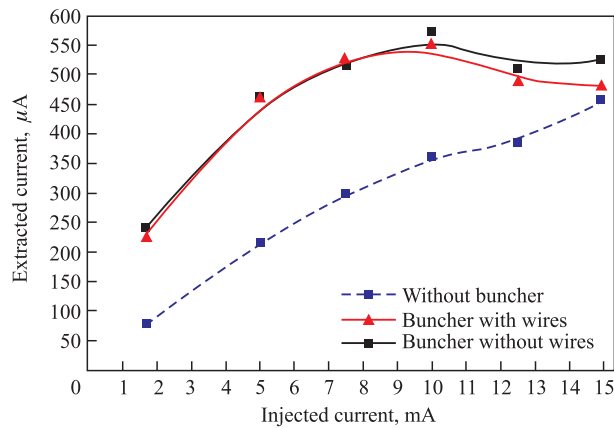
Fig. 15. Extracted beam current vs. the injected beam intensity
