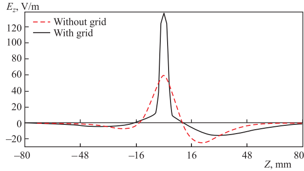
Fig. 14. E_z component vs. the Z coordinate
