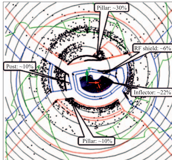
Fig. 22. Particle loss distribution in the central region
