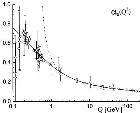
Fig. 1. Summary of BS+APT extracted ( \diamond ) and high energy ( \circ ) data for \alpha_s(Q^2) against the three-loop analytic running coupling (solid curve) and its perturbative counterpart (dashed curve) both normalized at the Z_0 boson mass.
