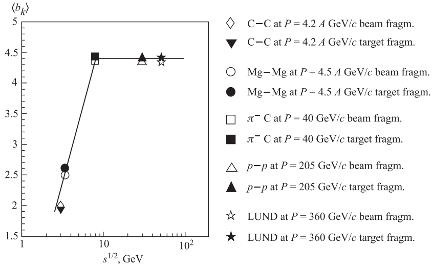
Fig. 4. Cluster width versus incident energy for different nuclear reactions
