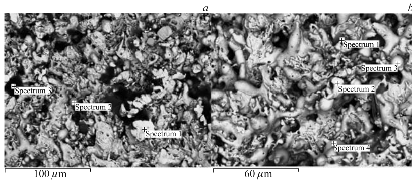
Fig. 18. SEM images of palladium specimen irradiated by \gamma -quanta
