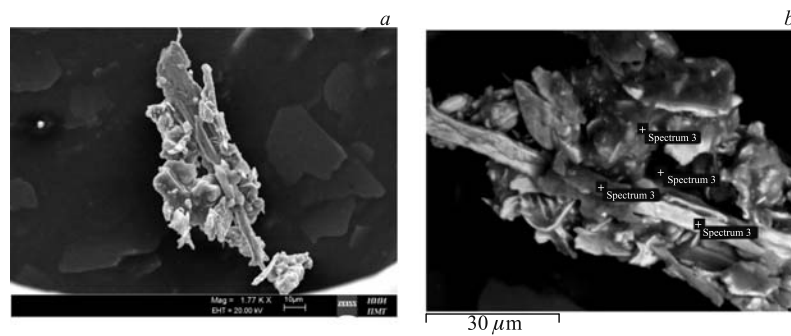
Fig. 11. a ) Complex microstructure on the «crater» floor, largely composed of brass. b ) SEM image of recrystallized complex structure largely composed of brass (Cu, Zn)
