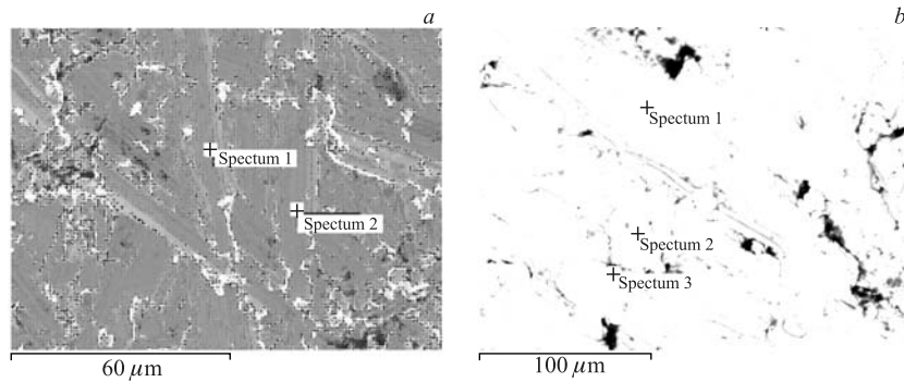
Fig. 20. SEM images of side surfaces of virgin ( a ) and irradiated by \gamma -quanta ( b ) Pd specimens
