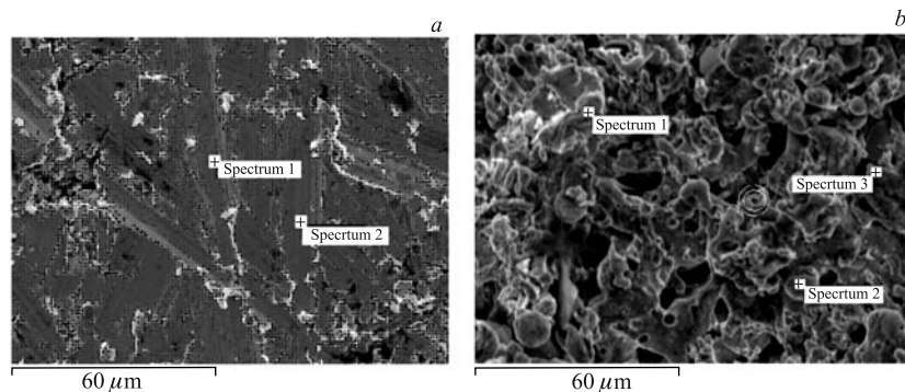
Fig. 17. SEM images of the ends of virgin (a) and irradiated by \gamma -quanta (b) palladium specimens
