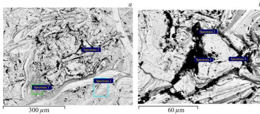
Fig. 22. Structure and element analysis of input beryllium bronze «window» plug
