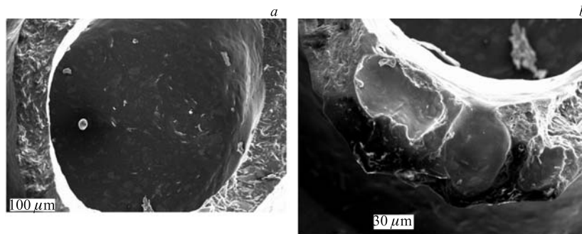
Fig. 9. Image of the «crater» with smooth walls and even edge ( a ) and patch of the «crater» wall with molten and congealed drops ( b )
