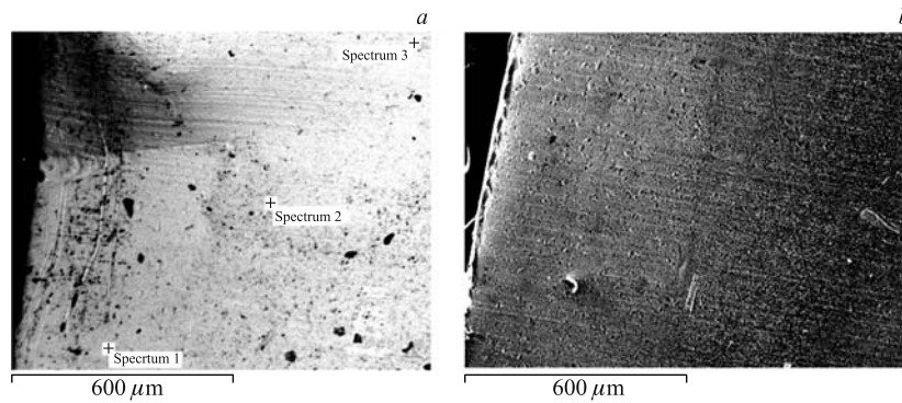
Fig. 16. SEM image of the split separating foil from the side facing inside the chamber ( a ) and the other side ( b ) adjacent to the loading brass screw
