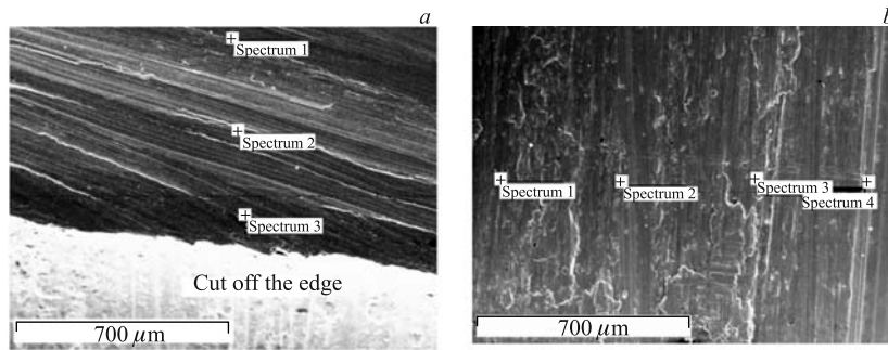
Fig. 21. SEM images of surface patches near the cut ( a ) and away from the split area of the brass sleeve ( b )
