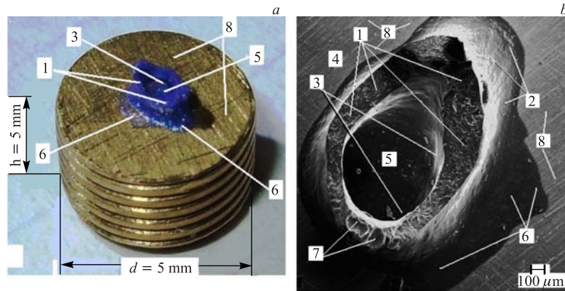
Fig. 5. a ) A photo of the brass screw (Fig.1, position 12) with the synthesized novel structure (SNS) and b ) image with the structure made by scanning electron microscopy (top view). The following designations are used in the photos: 1 — upper part of walls of «volcanic» structure with «crater»; 2 — shallow walls of SNS; 3 — smooth side walls of «crater»; 4 — brass screw surface; 5 — «crater» floor with structures of various compositions; 6 — molten and spread over surface «lava» from «crater»; 7 — molten and hardened clusters of SNS material; 8 — brass screw surface
