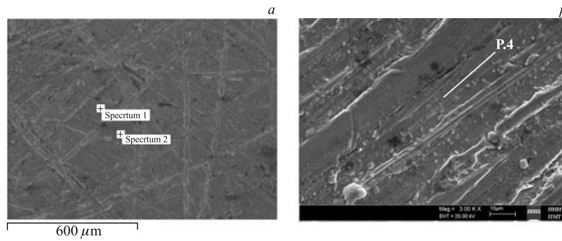
Fig. 15. a) SEM image of the virgin brass from which the brass screw is fabricated and b) surface of the brass screw near the SNS structure
