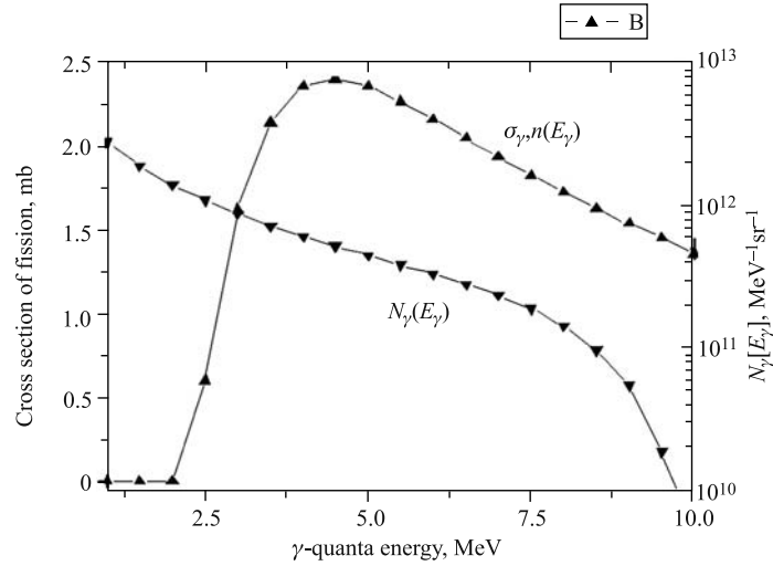
Fig. 2. Cross section of deuteron photodecay \sigma_{d(\gamma,n)p} (barn) and spectrum of \gamma -quanta N_\gamma(E_\gamma) ( \text{MeV}^{-1} \text{sr}^{-1} ) versus energy
