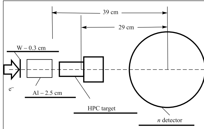
Fig. 4. The scheme of braking W-target, Al-absorber, high-pressure chamber (HPC), and neutron detector with a moderator during neutron yield measurements
