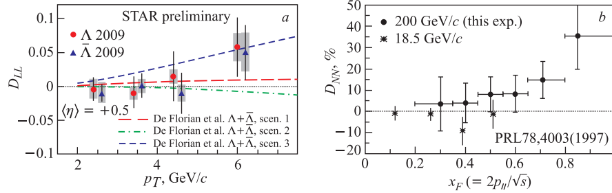
Fig. 6. Longitudinal D_{LL} and transverse D_{NN} transfer coefficients [4, 24]
