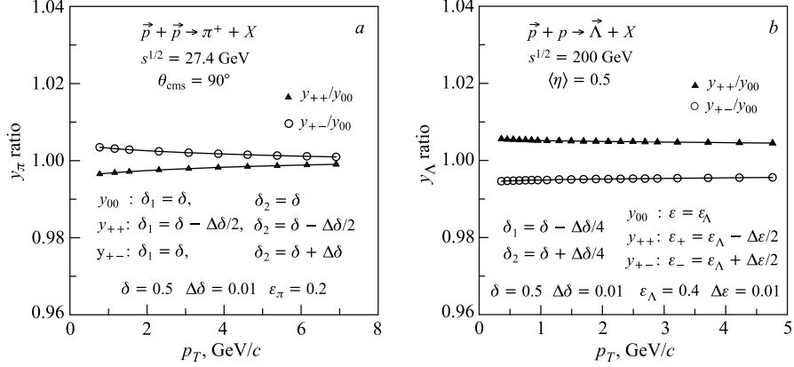
Fig. 9. Spin-dependent momentum fractions y_\pi, y_\Lambda as a function of the transverse momentum p_T and collision energy \sqrt{s} for processes \vec{p} + \vec{p} \rightarrow \pi^+ + X and \vec{p} + p \rightarrow \vec{\Lambda} + X
