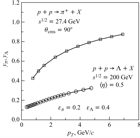
Fig. 8. Momentum fractions y_\pi and y_\Lambda as a function of the transverse momentum p_T and collision energy \sqrt{s} for the processes p + p \rightarrow \pi^+ + X at \sqrt{s} = 27.4 GeV and p + p \rightarrow \Lambda^0 + X at \sqrt{s} = 200 GeV, respectively
