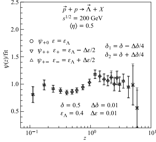
Fig. 7. The scaled spin-dependent \Psi_{++} , \Psi_{+-} and spin-independent \Psi_{00} functions for \Lambda hyperon production in p + p collisions at \sqrt{s} = 200 GeV and \langle\eta\rangle = 0.5 in z -presentation
