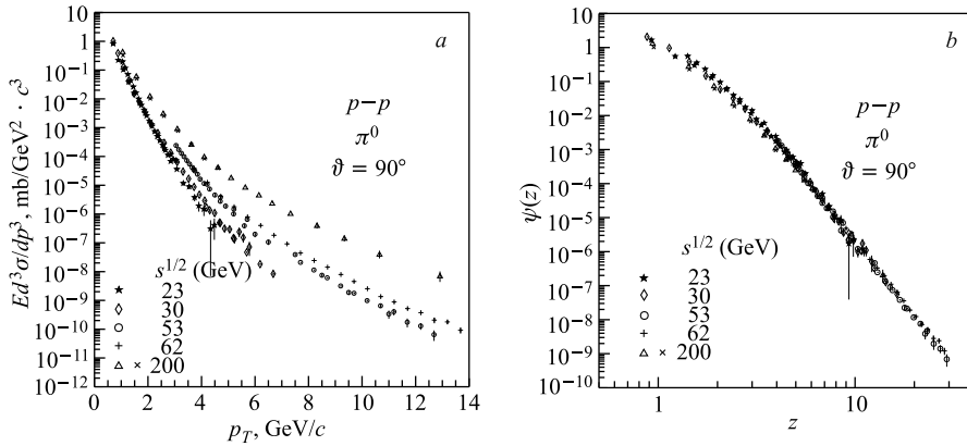
Fig. 3. Spectra of the pion production in the proton-proton collisions at \sqrt{s} = 23-200 GeV and \vartheta_{\text{cms}} = 90^\circ in (a) p_T - and (b) z -presentations [12, 13]
