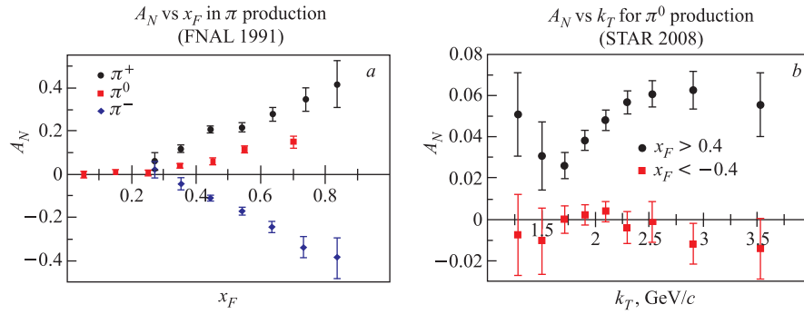
Fig. 2. The pion single transverse spin asymmetry A_N ( a ) as a function of Feynman x_F reported by the E581 and E704 collaborations for 0.7 < k_T < 2.0 GeV/c, and ( b ) as a function of the pion transverse momentum k_T collected by the STAR collaboration. Plots are taken from [22]
